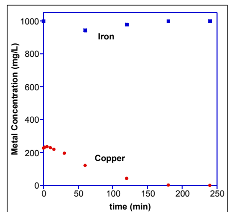
Copper removal from a mixture of copper and iron, pH 2.3 H 2 SO 4 electrolyte, batch process.
